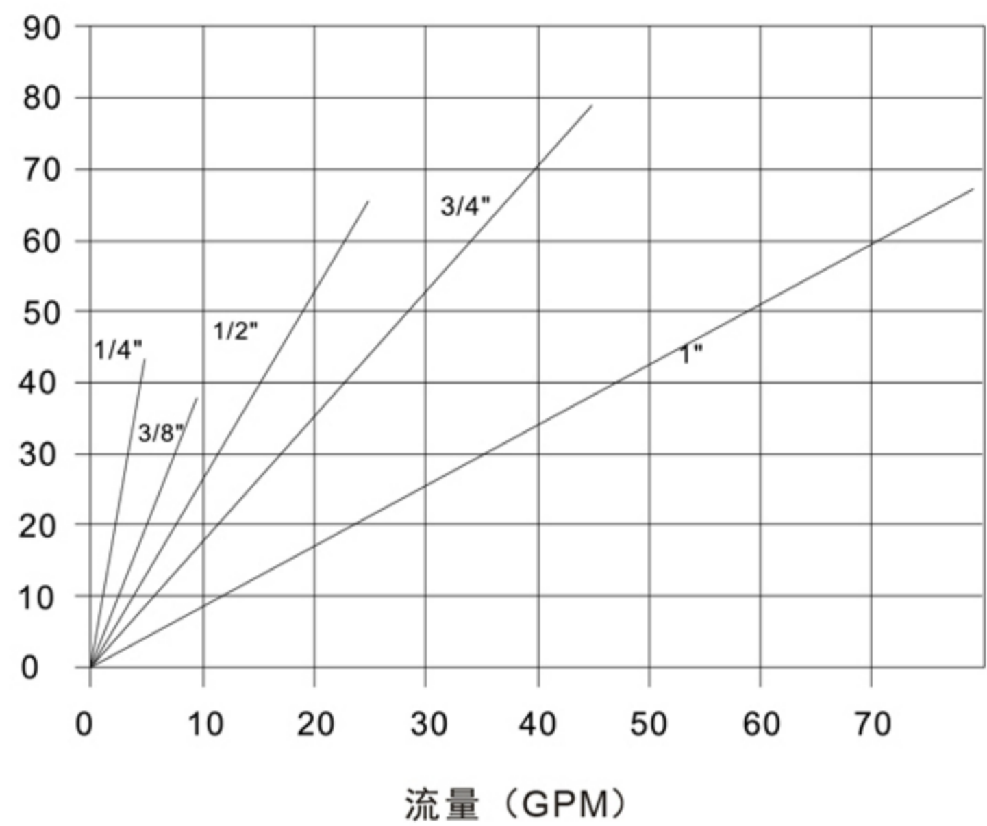
压降 Pressure Drop-in PSID
